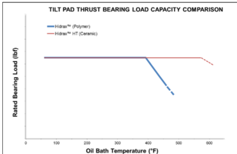
Load capacity at increasing temperatures for polymer Hidrax versus ceramic Hidrax HT center pivot TPT bearings
