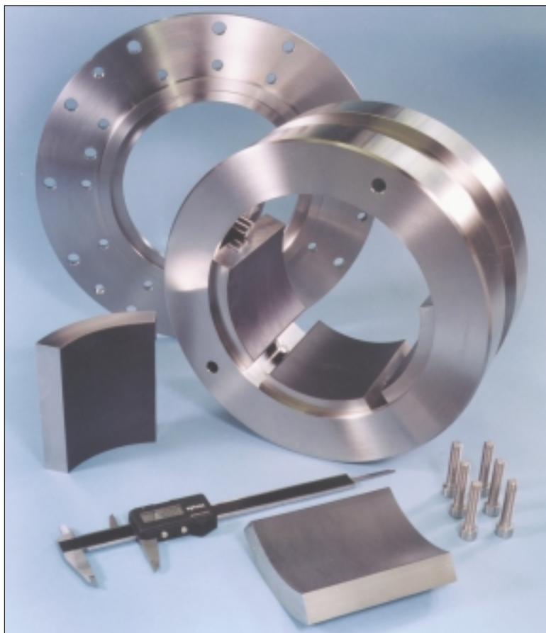
Fig. 1. Polymer-lined radial bearing for operation with amine as the lubricant.
